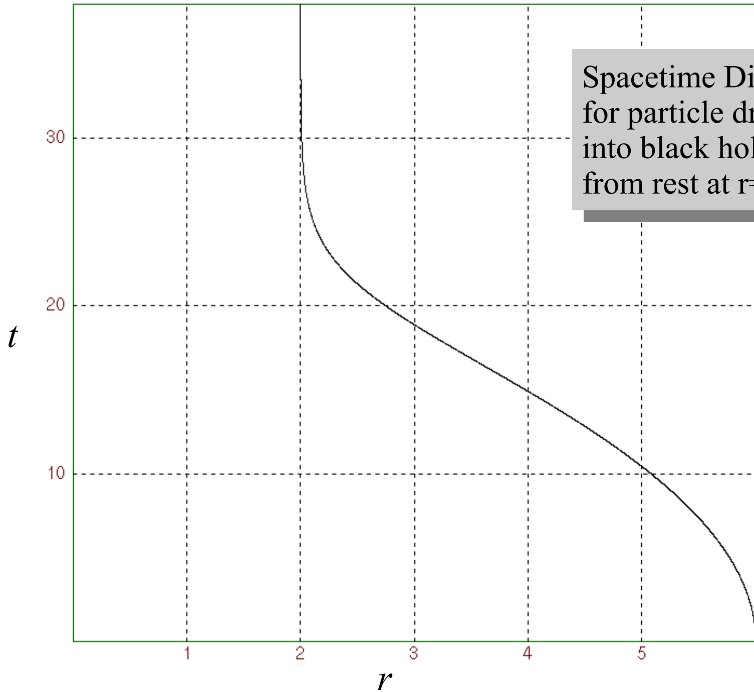
(Schwarzschild coordinates)
