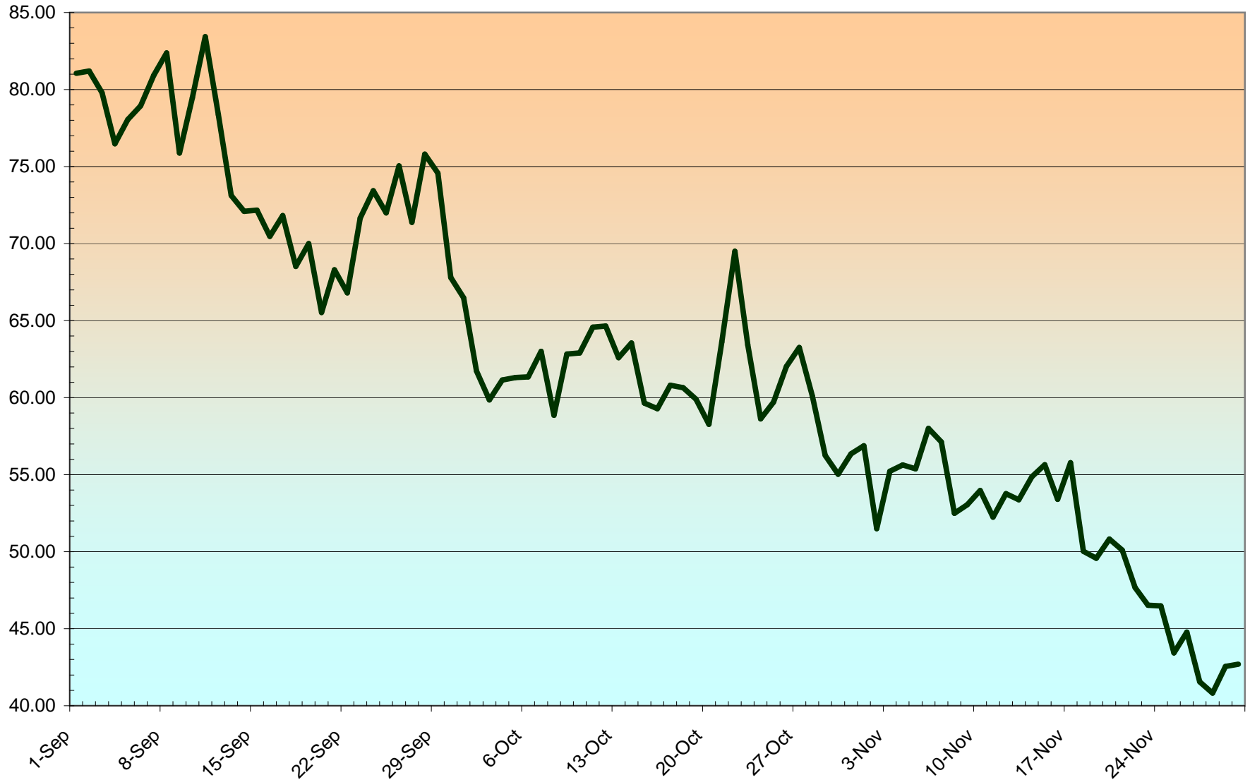
The Average Autumn High Temperature Plunge at Rod's House Since 2005
