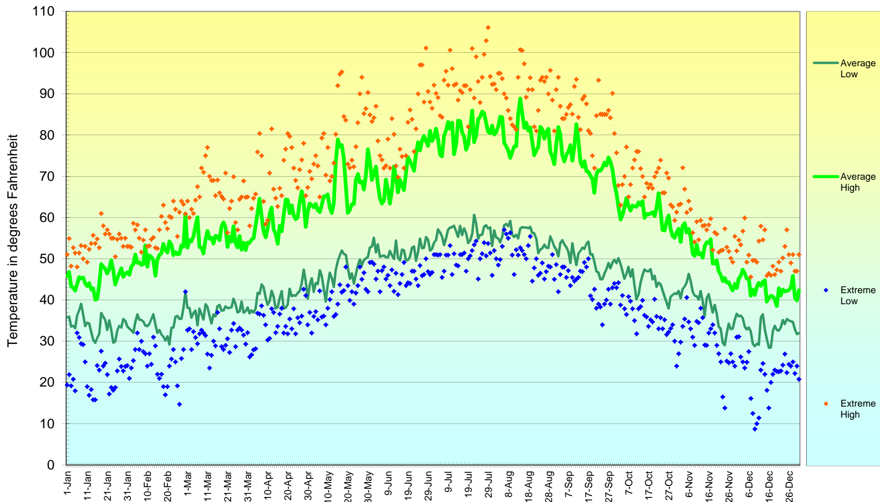
Rolling Average Temps East Vancouver, WA : With Extremes ( 2005 - current)
