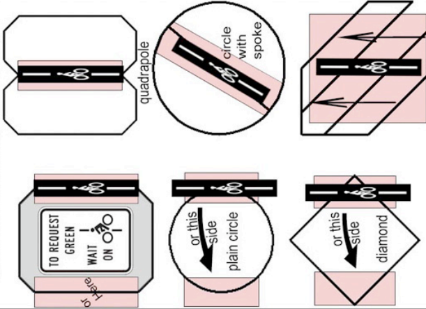
Typical traffic detecting induction loops:
